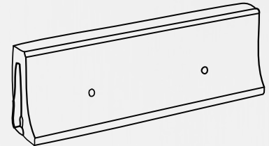
PIER BARRIER (CPB) 2500 L x 810 H x 414 W
