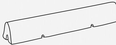
LOW BARRIER (CLB-1) 3000 L x 457 H x 457 W
