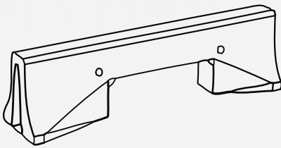
DRAINAGE BARRIER (CDBE) 2500 L x 690 H or 810 H x 550 W
