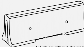
MEDIAN BARRIER (CMB) 2500 L x 810 H x 600 W
