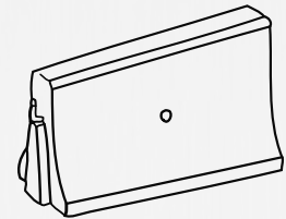
TRANSITION BARRIER (CTB-2) 1300 L x 810 H x 600 W
