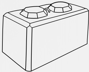
STANDARD BLOCK 1500 L x 750 W x 750 H
