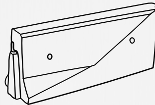
TRANSITION BARRIER (SBPT) 2500 L x 810 H x 600 W
